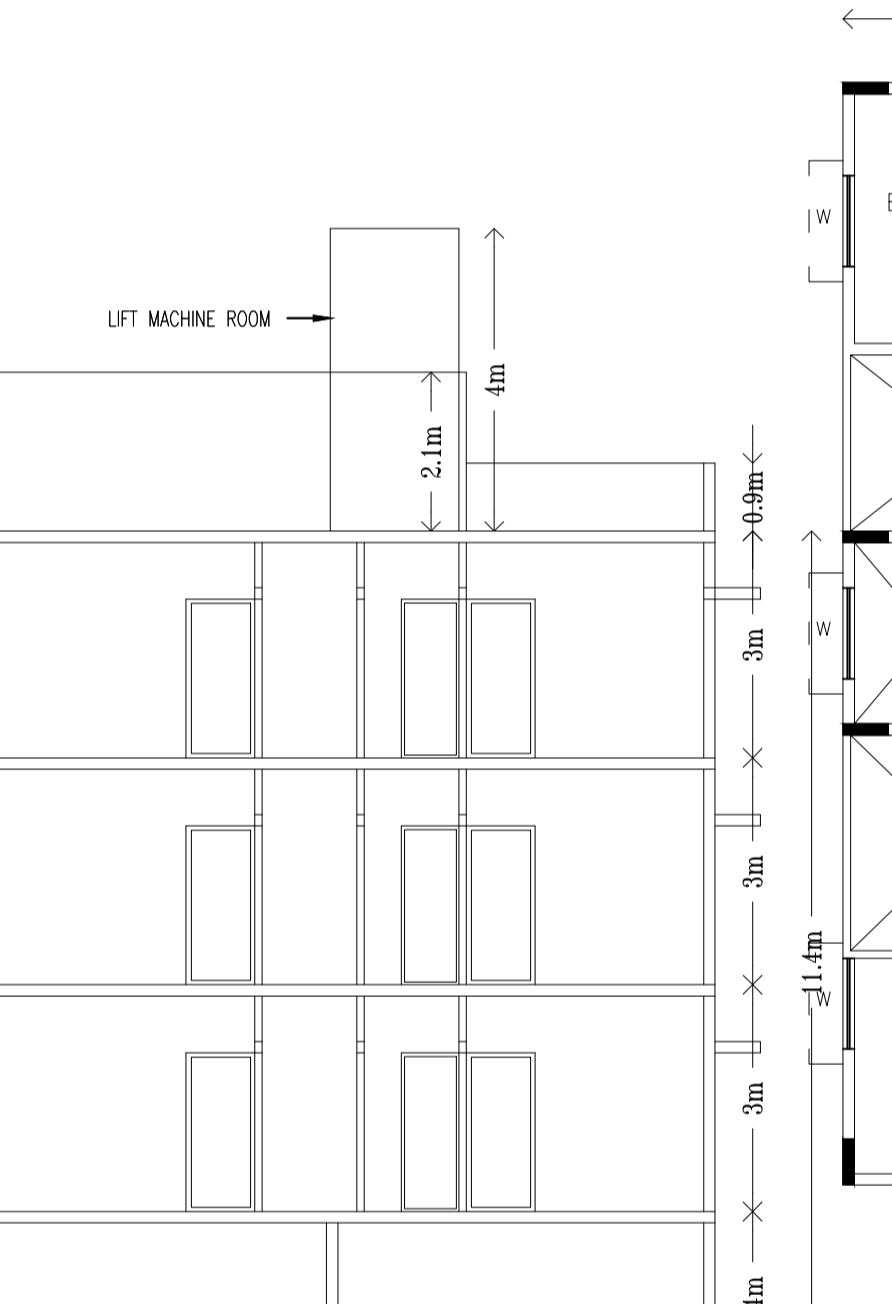
SECTION @ X-X
